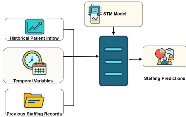
FIGURE 3. LSTM-based forecasting architecture utilizing historical inflow, temporal features, and past records to generate department-wise staffing predictions.
