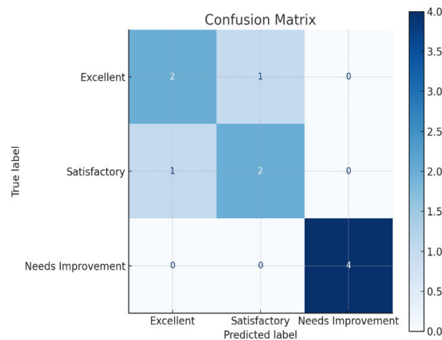
FIGURE 15. Confusion matrix illustrating classification results for performance categories—Excellent, Satisfactory, and needs improvement—demonstrating model accuracy and misclassification patterns.
