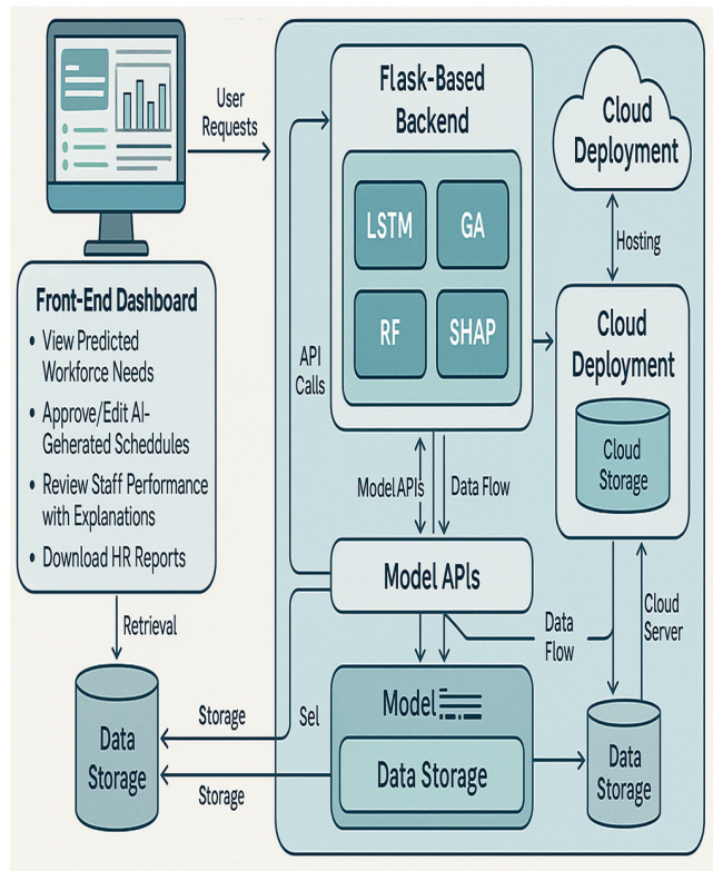
FIGURE 7. System architecture of the AI-HRMS, illustrating the integration of front-end dashboard, Flask-based backend (LSTM, GA, RF, SHAP), model APIs, and cloud deployment for real-time workforce management.
