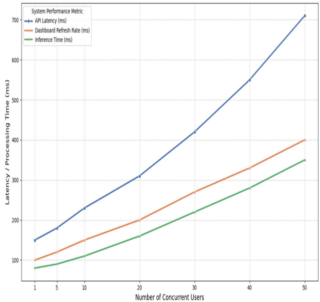
FIGURE 20. System performance trends showing increased API latency, dashboard refresh time, and inference time as concurrent users rise.
