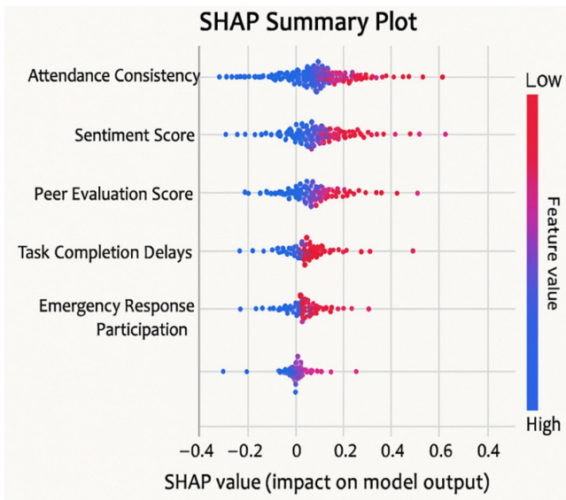
FIGURE 17. SHAP summary plot showing key features impacting model output. Attendance consistency and sentiment score had the most significant influence.
