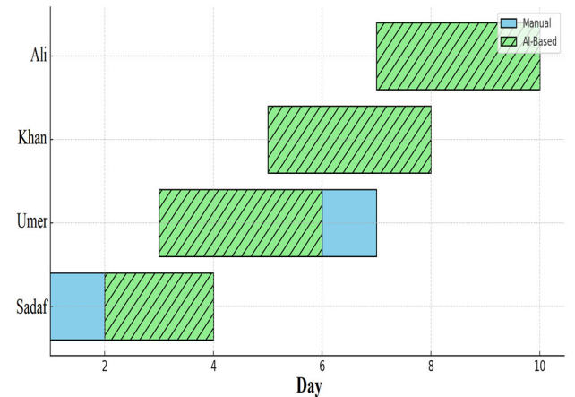
FIGURE 13. Comparative Gantt chart illustrating manual versus AI-based shift allocations across staff members over a 10-day period, emphasizing improved coverage and efficiency with AI-generated schedules.
