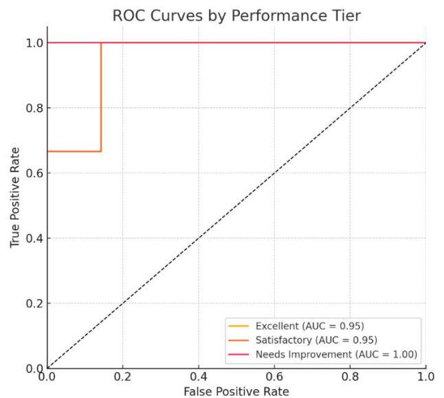
FIGURE 16. ROC curves for performance tiers with AUC scores: Excellent (0.95), Satisfactory (0.95), and Needs Improvement (1.00).
